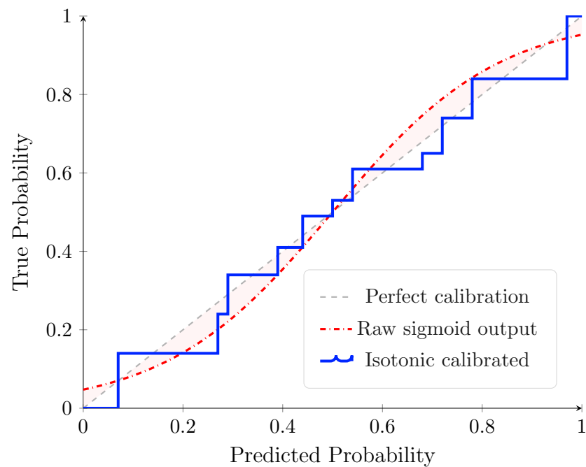
Isotonic Calibration of Meta-Learner
